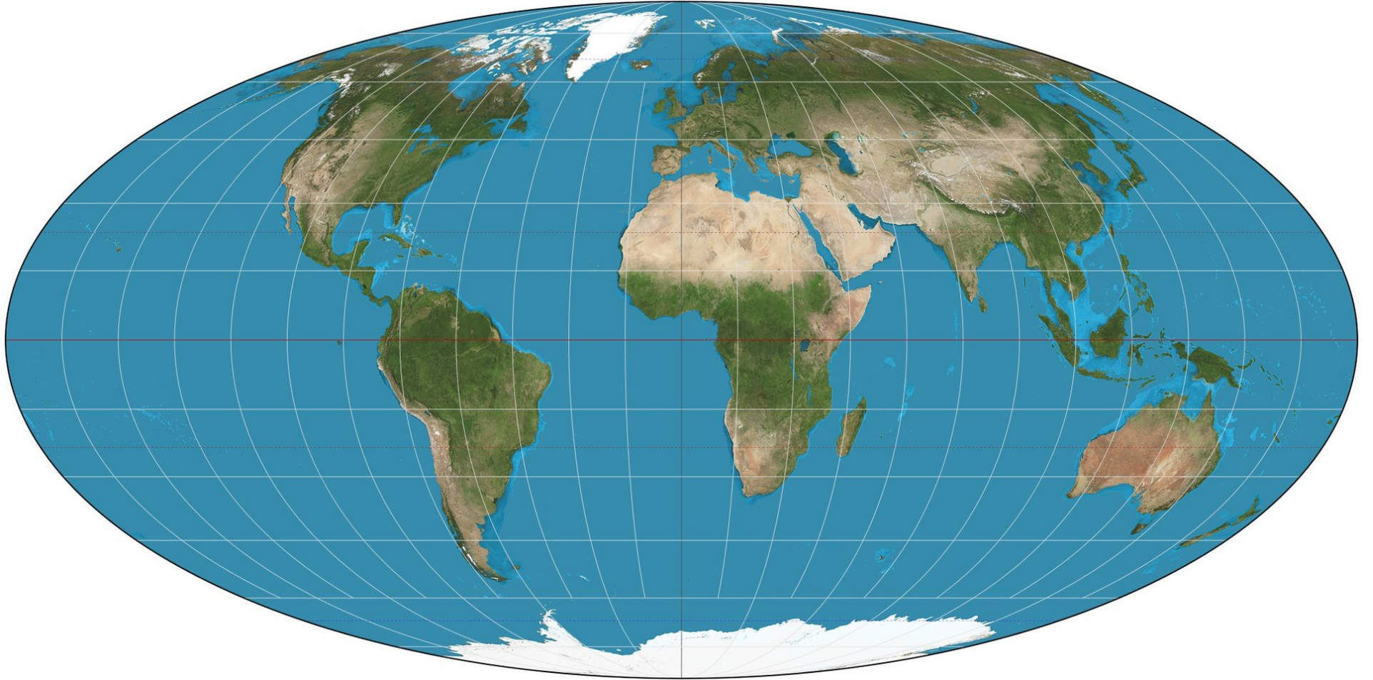
Mollweide projection
