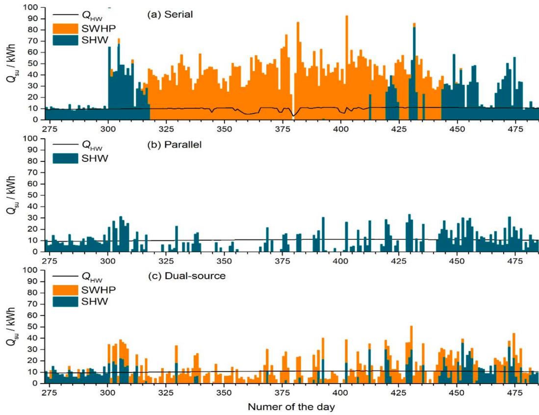
Fig. 11. Variations of daily solar thermal energy used for SH and HW over a heating season.
