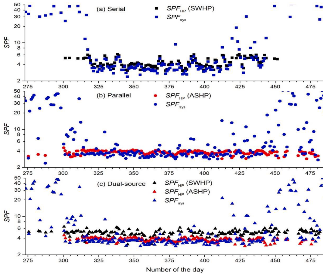
Fig. 14. Variations of daily SPF_{sys} and SPF_{HP} over a heating season.
