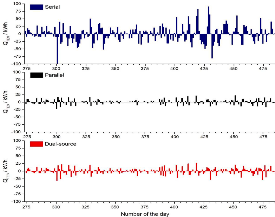
Fig. 12. Variations of daily thermal energy storage ( Q_{TES} ) over a heating season. Positive value refers to the thermal energy charged and negative value refers to the thermal energy discharged.
