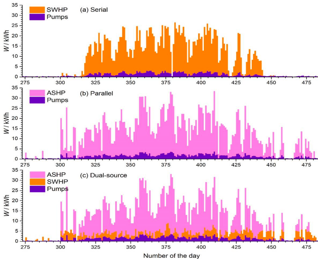
Fig. 10. Variations of daily electricity consumed by the systems over a heating season.
