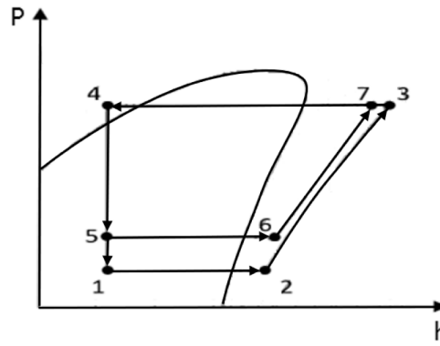
Fig. 6. P - h diagram of ideal vapour-compression cycle HPs.
