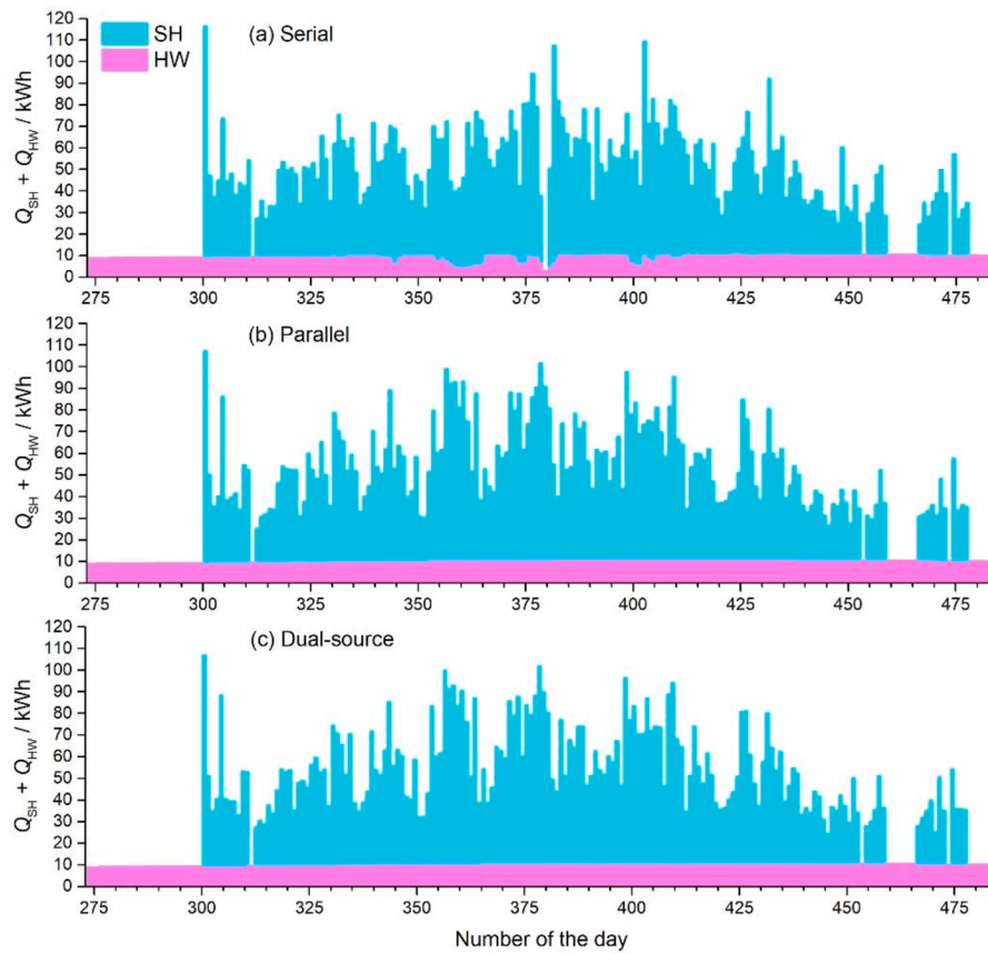
Fig. 8. Variations of daily heat provision for SH and HW for three systems over a heating season.
