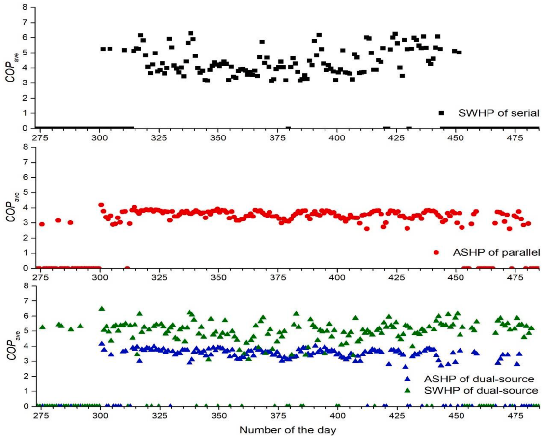
Fig. 13. Variations of daily averaged COP of the HPs in three systems over a heating season.
