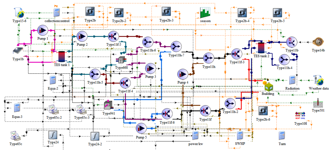
c) Dual-source IX-SAASHP
