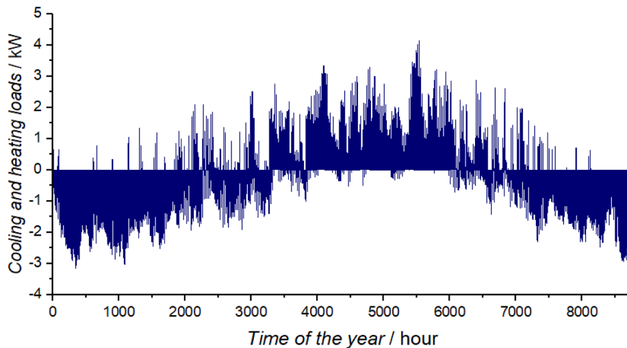
Fig. 1. Hourly cooling (positive) and heating (negative) loads of the house SFH 45 at room air temperature T_{\text{room}} of 18 °C over a typical year of weather conditions in London.
