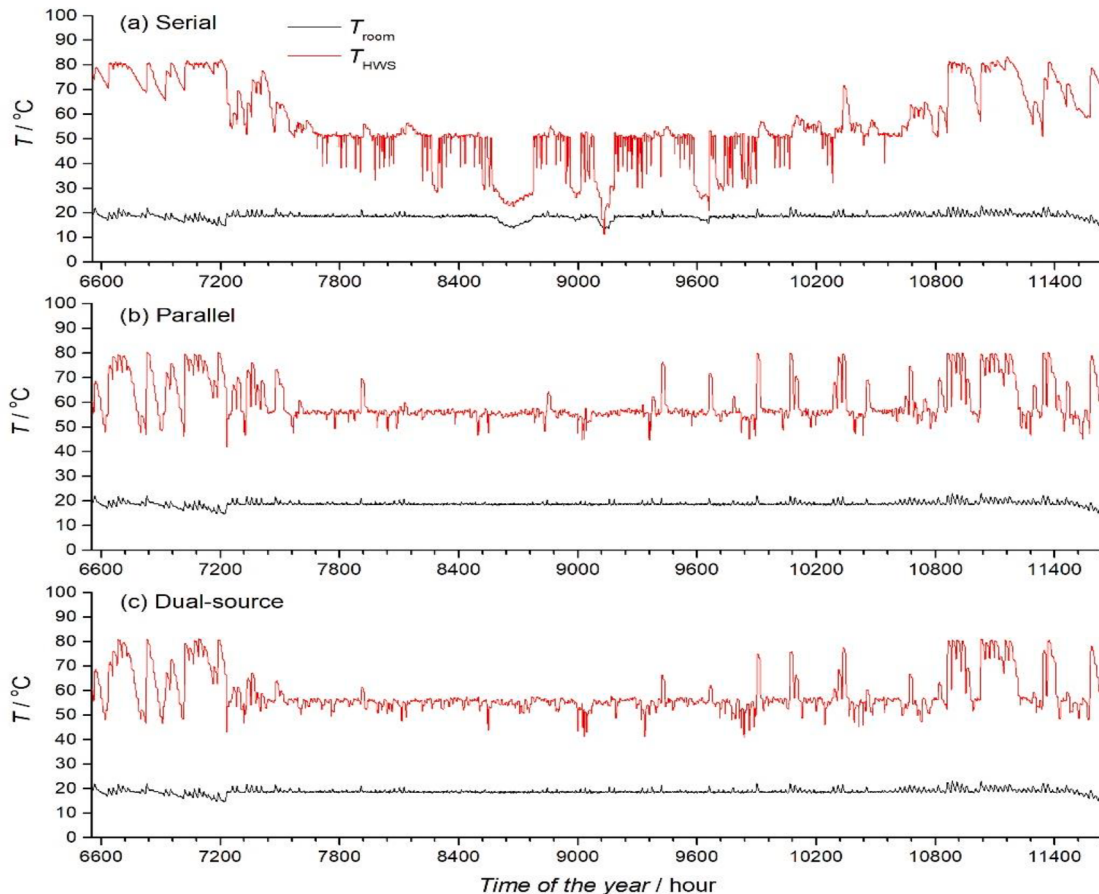
Fig. 7. Variations of room air temperature and HW temperature at the outlet of TES tank 2 for three systems over a heating season.
