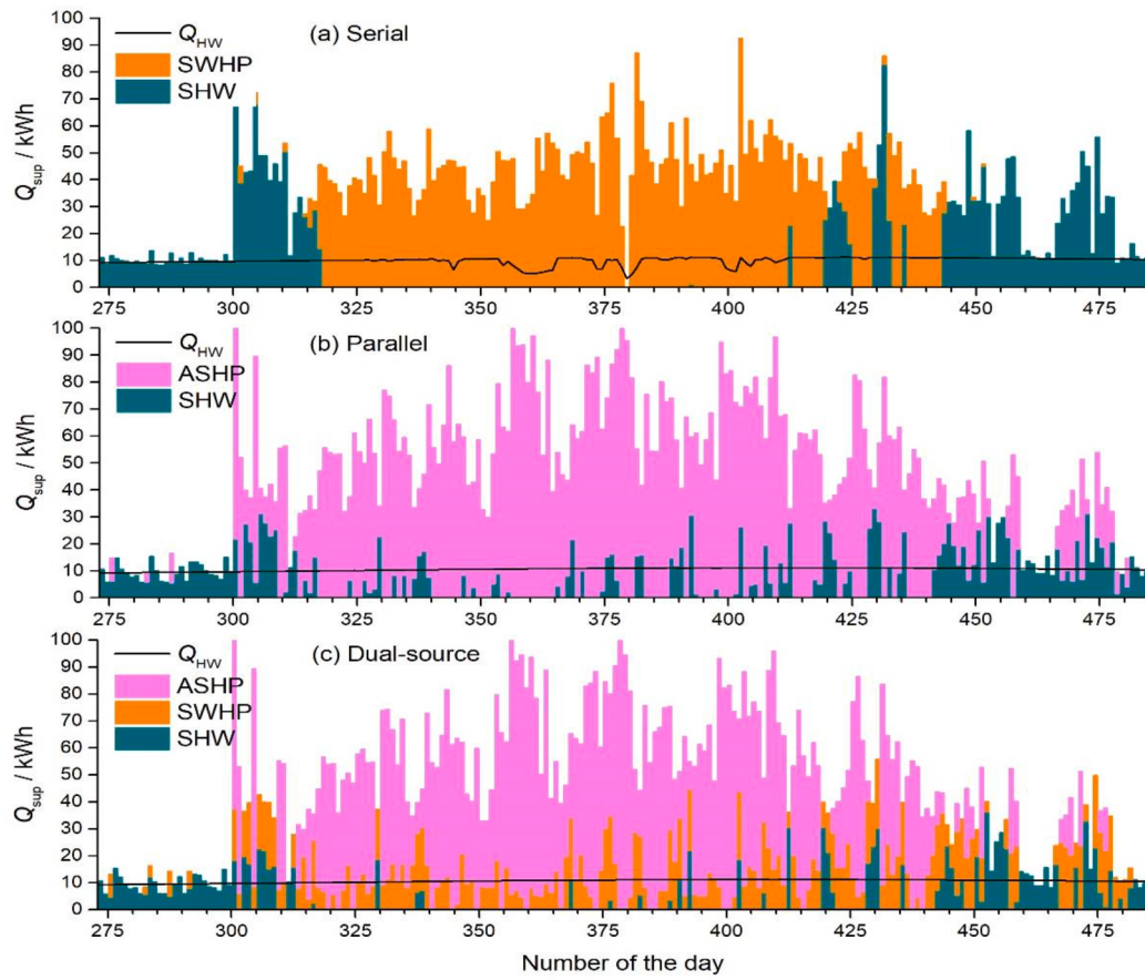
Fig. 9. Variations of daily heat provision supplied by direct SHW, ASHP and SWHP for three systems over a heating season.
