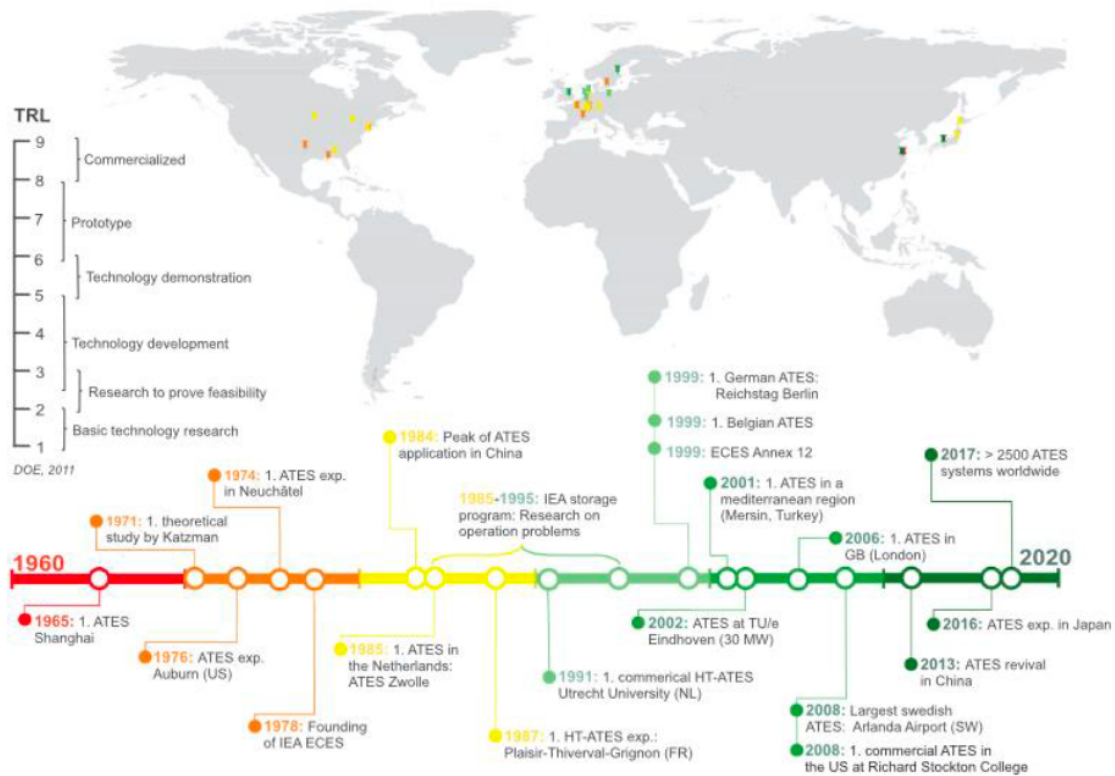
Figure 4 displaying ATES locations worldwide (Fleuchaus et al, 2018)
