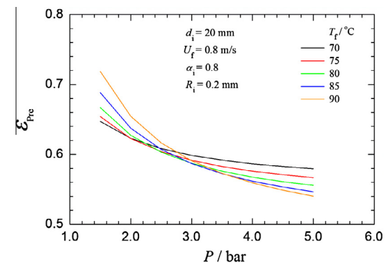
Fig. 14. Variation of predicted bubble size ratio with bulk liquid pressure for different bulk fluid temperatures.
