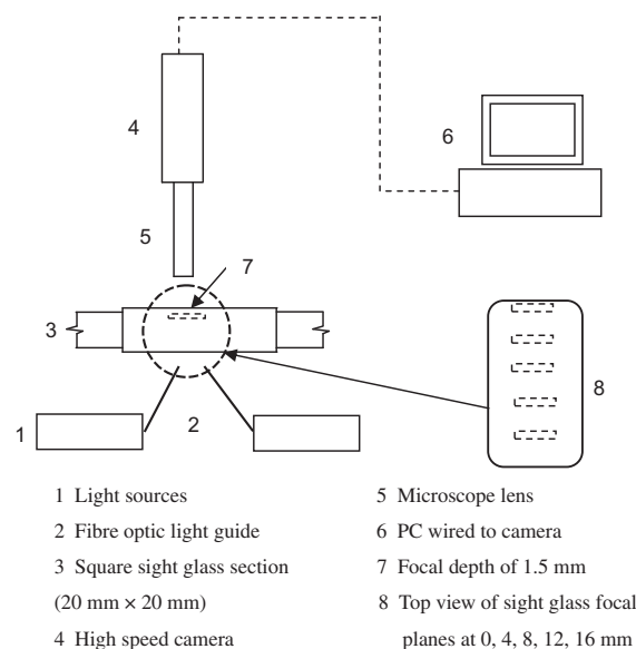
Fig. 3. Bubble size measurement equipment.
